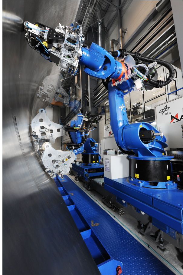
Figure 3: GroFi - realizing a combined usage of fiber placement and tape laying technology
