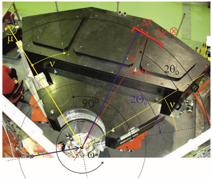
Figure 1: Flat-Cone Diffractometer E2, with the principle geometry axes. (© J.-U. Hoffmann, HZB)
