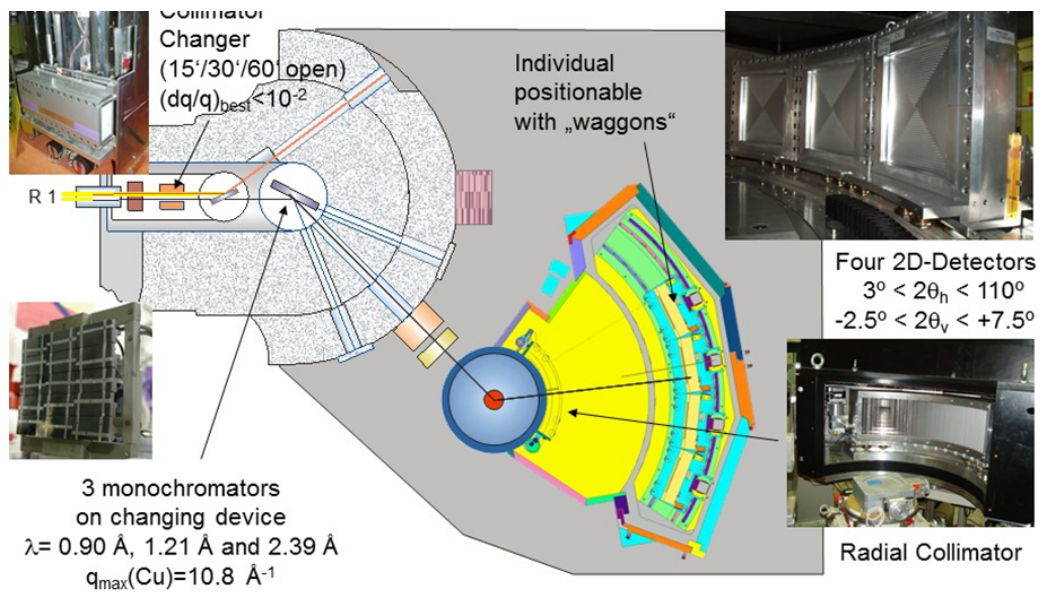
Figure 2: Schematic sketch of E2.
